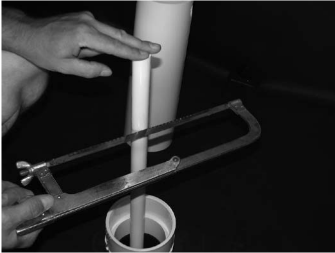
Step 7 Using a hacksaw, cut off the \frac{3}{4} " (1.90cm) fill line at the mark you made earlier.
